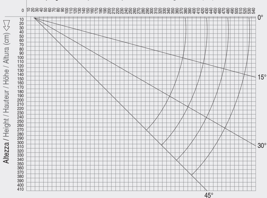
Utfallsdiagram
